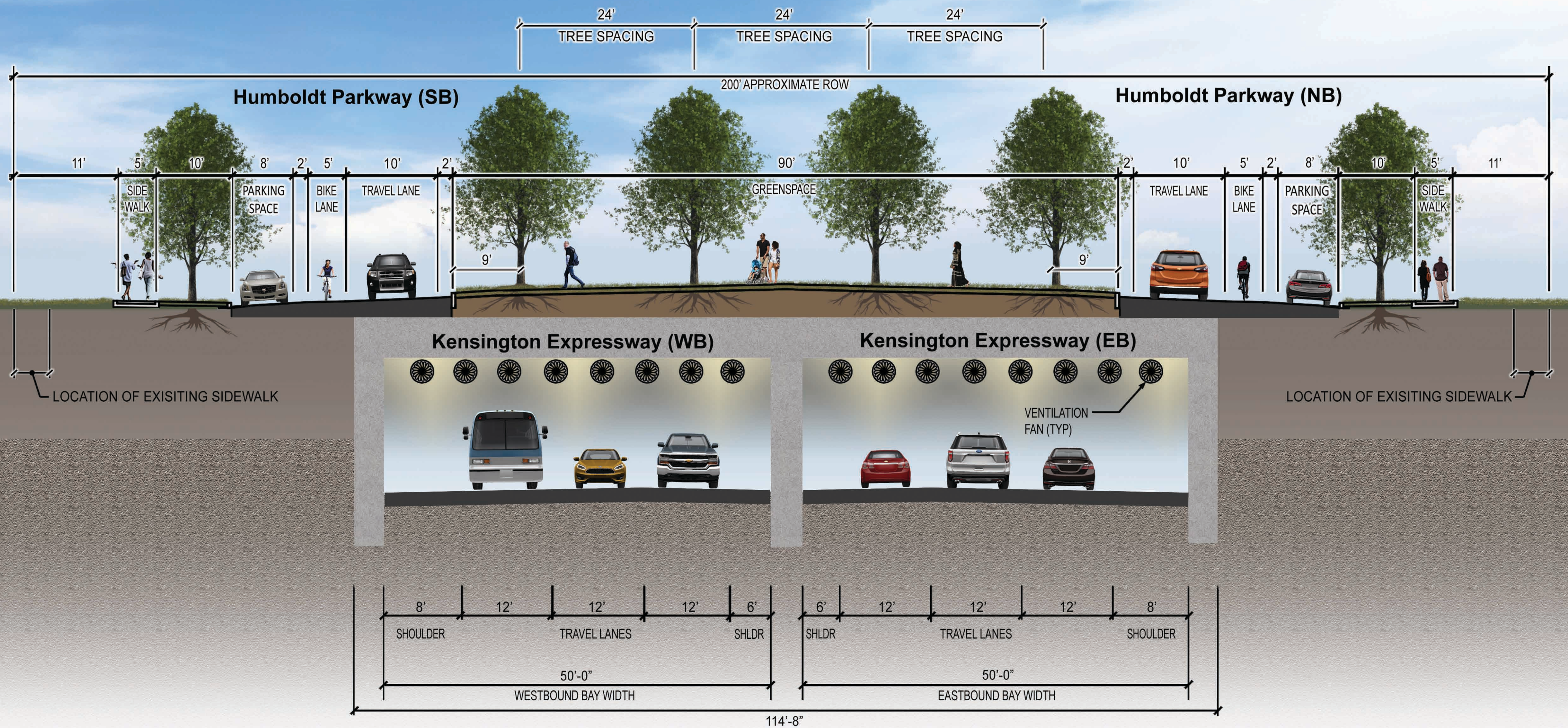
SECTION H-H PROPOSED CORRIDOR
