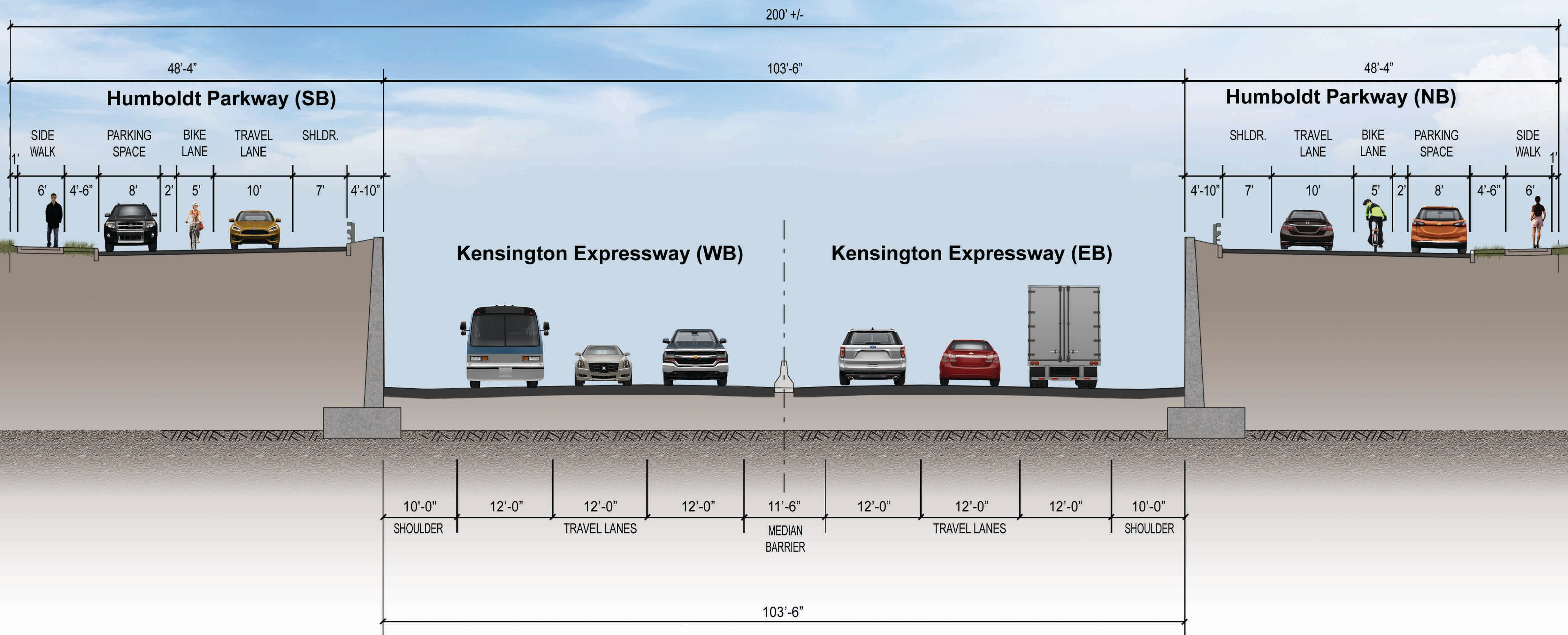
SECTION H-H EXISTING CORRIDOR
